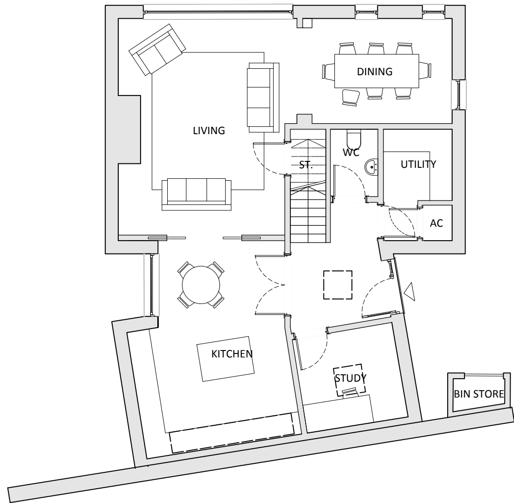
PLOT 1 - GROUND FLOOR PLAN
