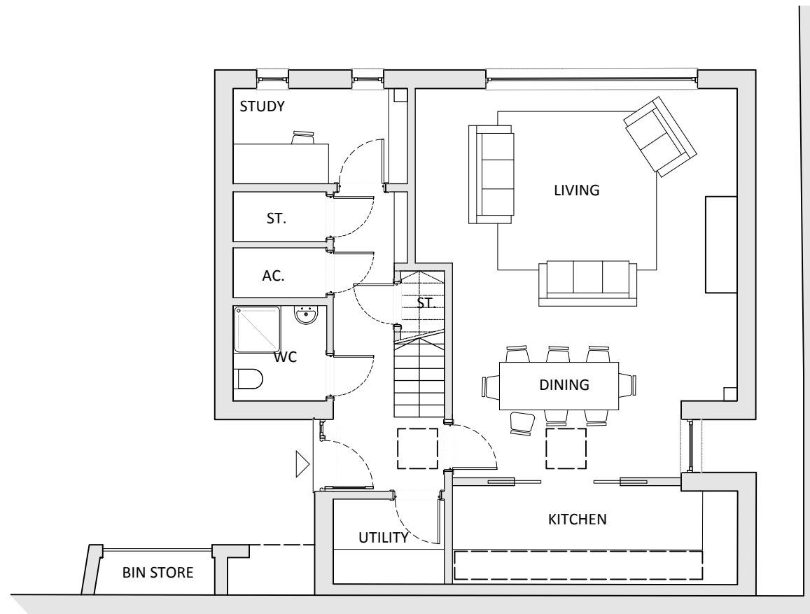
PLOT 2 - GROUND FLOOR PLAN
